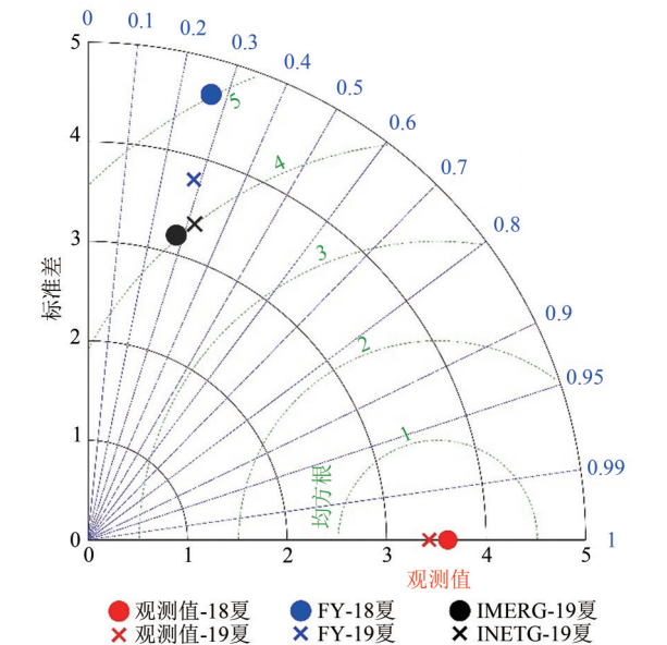
图2 2018年、2019年夏季3套产品统计性能泰勒图 Fig. 2 Taylor diagram of statistical performance for three datasets of products in the summers of 2018 and 2019
