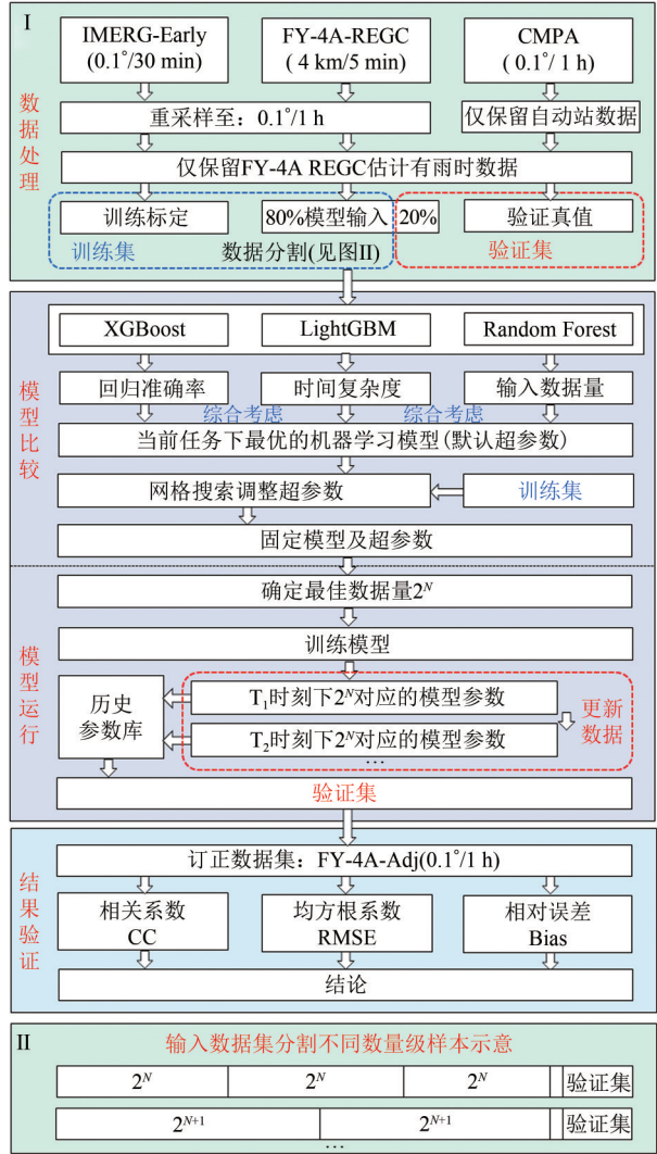
图1 基于集成学习的快速订正算法 Fig. 1 Fast correction algorithm based on ensemble machine learning
