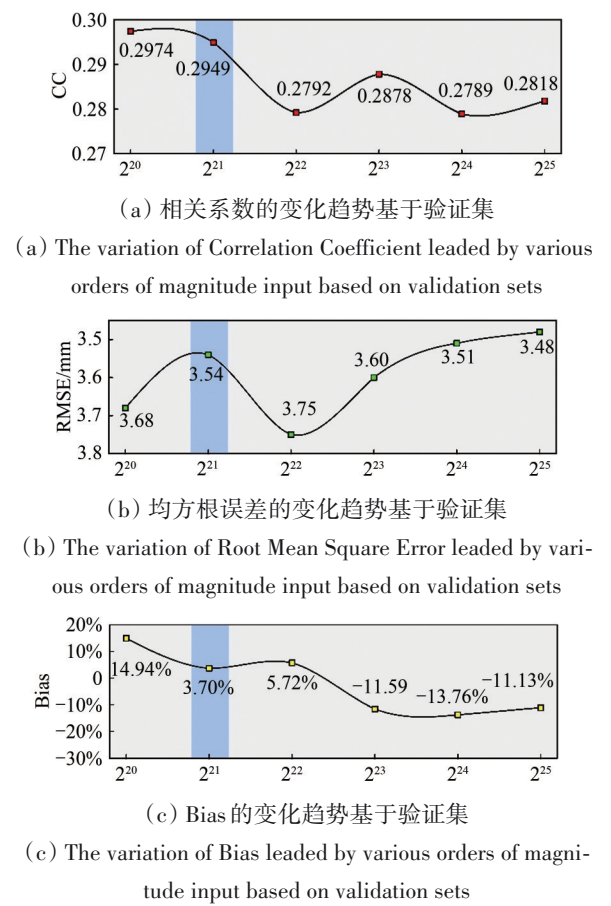
图5 各数量级输入导致评估结果(蓝色代表优选数据量) Fig. 5 Performance changing trends (The blue areas represent the best)
